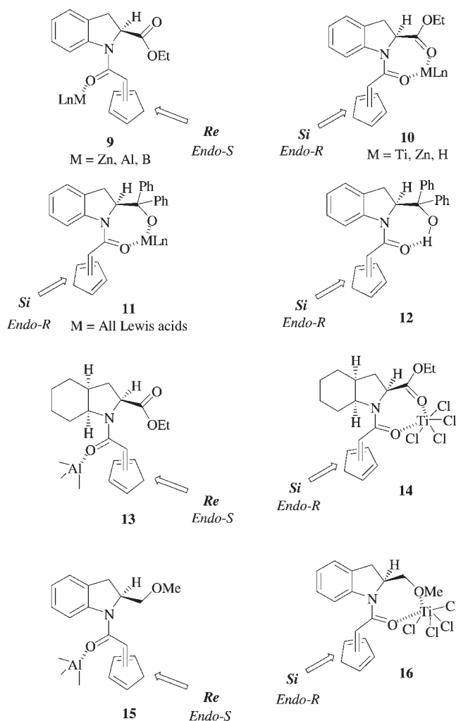
Figure 2. Mechanism of Diels–Alder cyclizations
