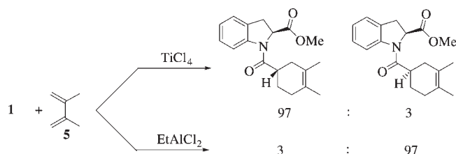
Figure 3. Diels–Alder cyclizations of 1 with 5
