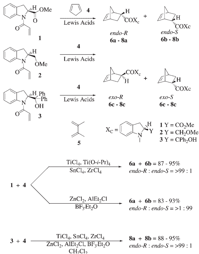
Figure 1. Diels-Alder cyclizations
