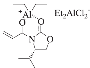
Figure 4. Evans' model dienophile
